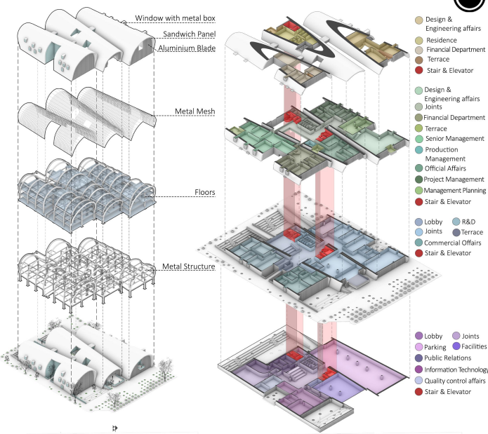
Exploded Diagram
