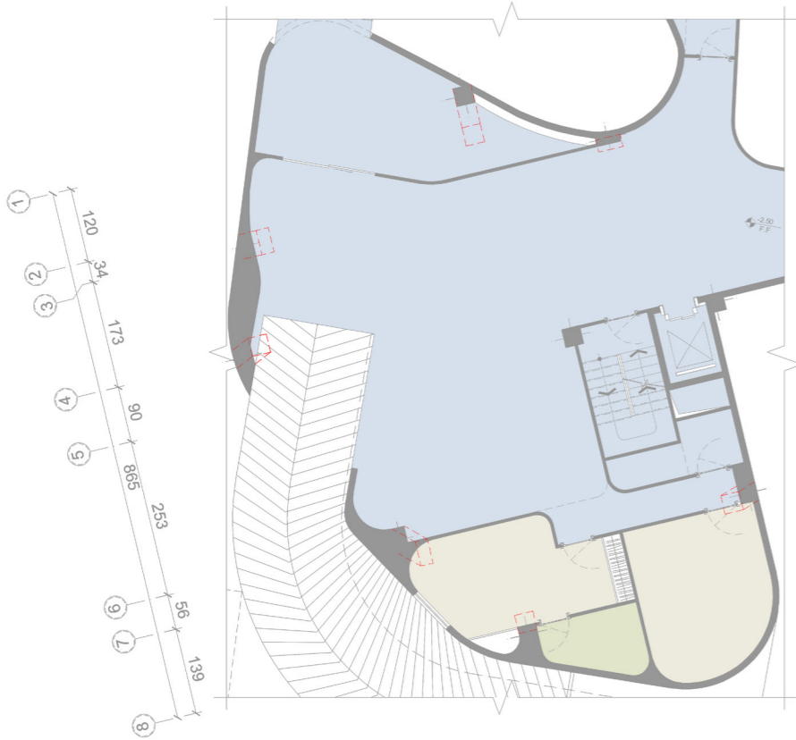
Private Section (Basement) Scale: 1/200
