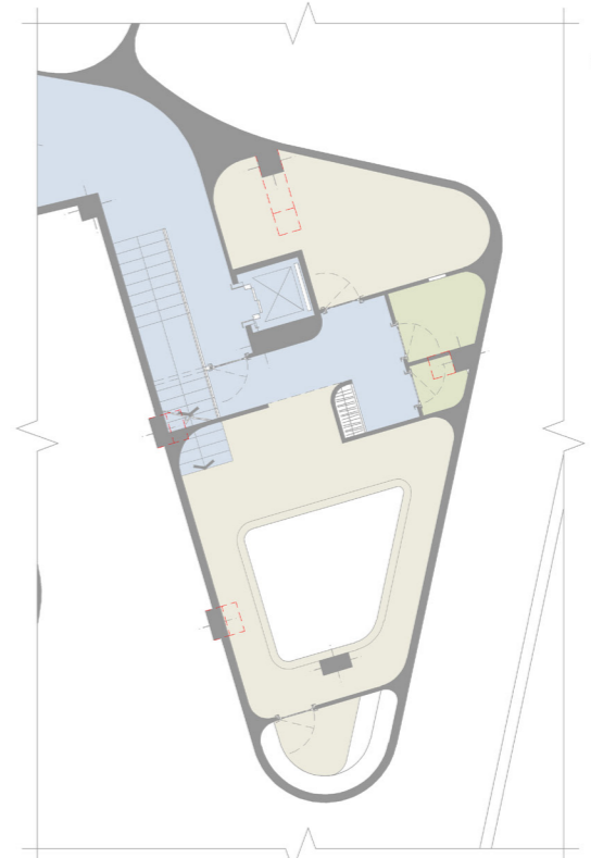
Services Section (Basement) Scale: 1/200
