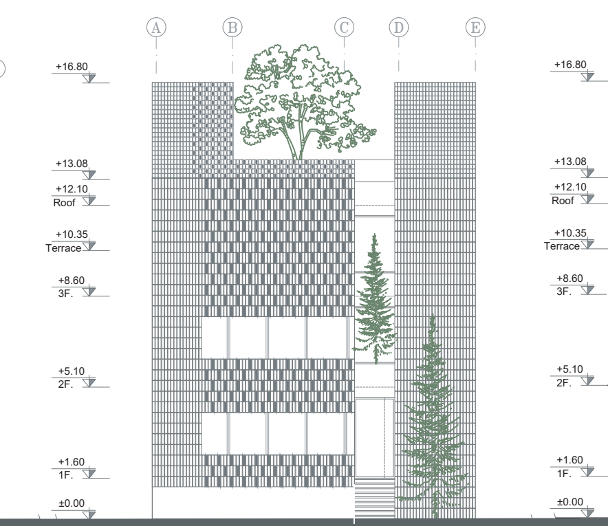
SOUTH ELEVATION 1:200
