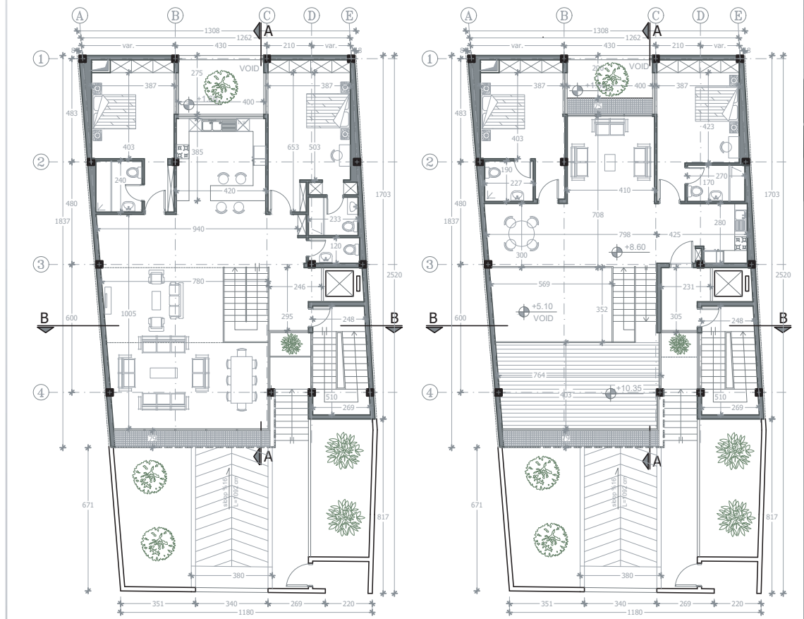
■ FIRST FLOOR IN DUBLEX PLAN 1:250
