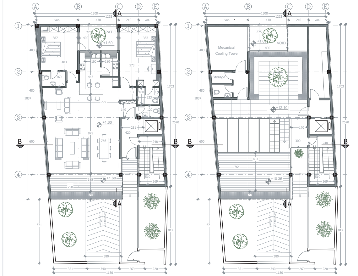
■ GROUND FLOOR PLAN 1:250
