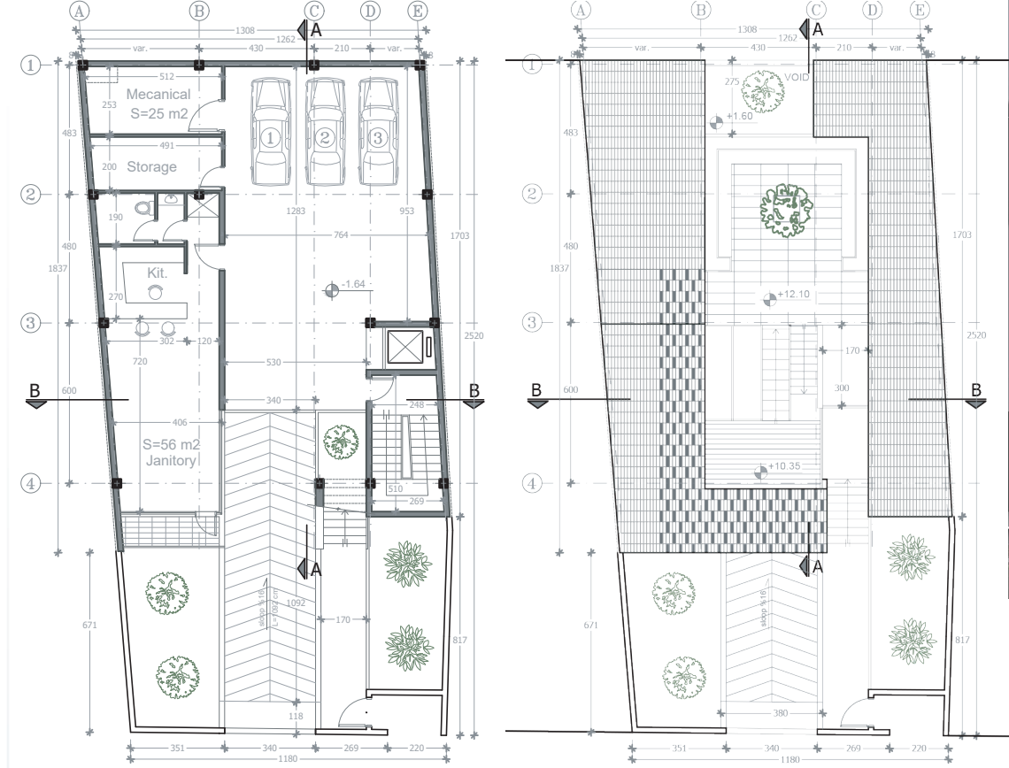
■ -1 st FLOOR PLAN 1:250
