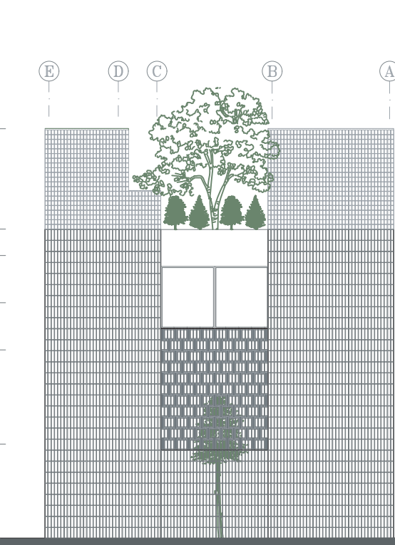
NORTH ELEVATION 1:200
