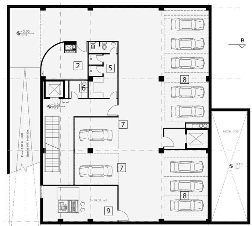
Plan Basement -1
