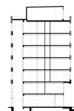
cross section B-B
