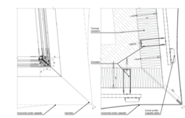
detail façade corner
