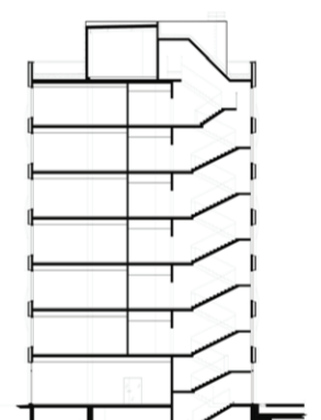
cross section C-C
