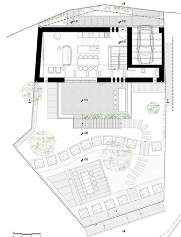
PLAN_ENTRANCE LEVEL
